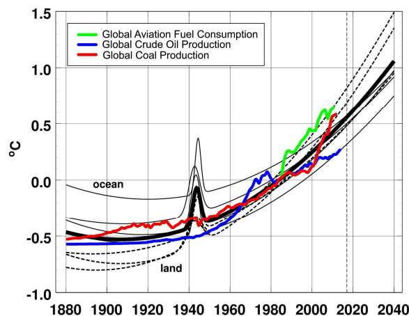
Fig. 2. Copy of Gottschalk's fitted curves for eight NOAA data sets showing relative temperature profiles over time [26] to which are added proxies for particulate pollution. has self-regulated itself thereby producing an environment favorable for the existence of life Dashed line: land; light line: ocean; bold line: weighted average. From [19]
