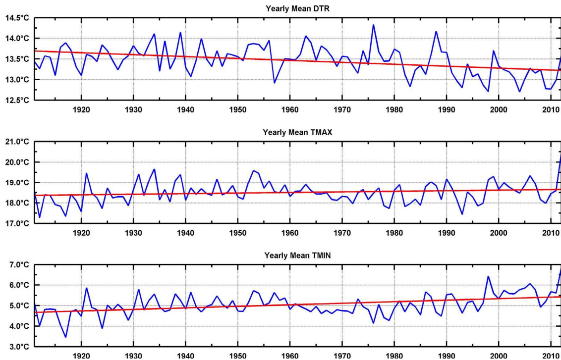
Fig. 1. Yearly mean DTR, T_{max} , and T_{min} over the continental USA. The red lines are linear regressions. From [11], ( http://creativecommons.org/licenses/by-nc-nd/3.0/ )
