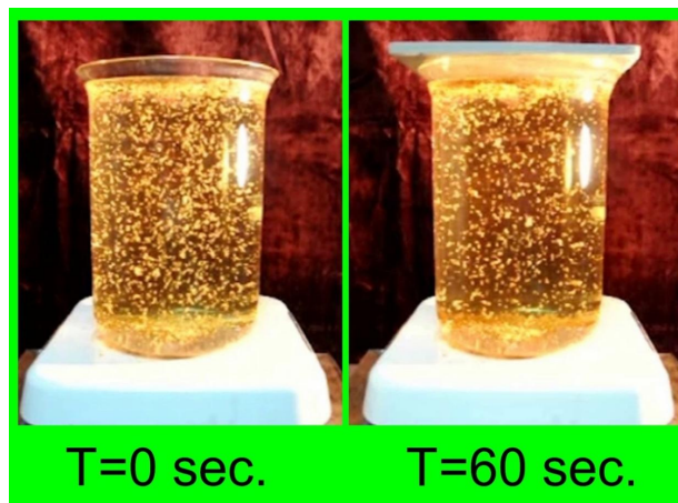
Fig. 3. From [22]. A beaker of water on a regulated hot plate with celery seeds pulled along by the fluid convection motions. Placing a ceramic tile atop the beaker a moment after T=0 reduced heat-loss, effectively warming the upper solution’s temperature, thus lowering the adverse temperature gradient, and reducing convection, indicated by the decreased number of celery seeds in motion at T=60 sec
