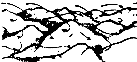
FIGURE 170. Windflow over various types of terrain. The many deviations from these patterns depend on wind speed, slope profile, and terrain roughness.
