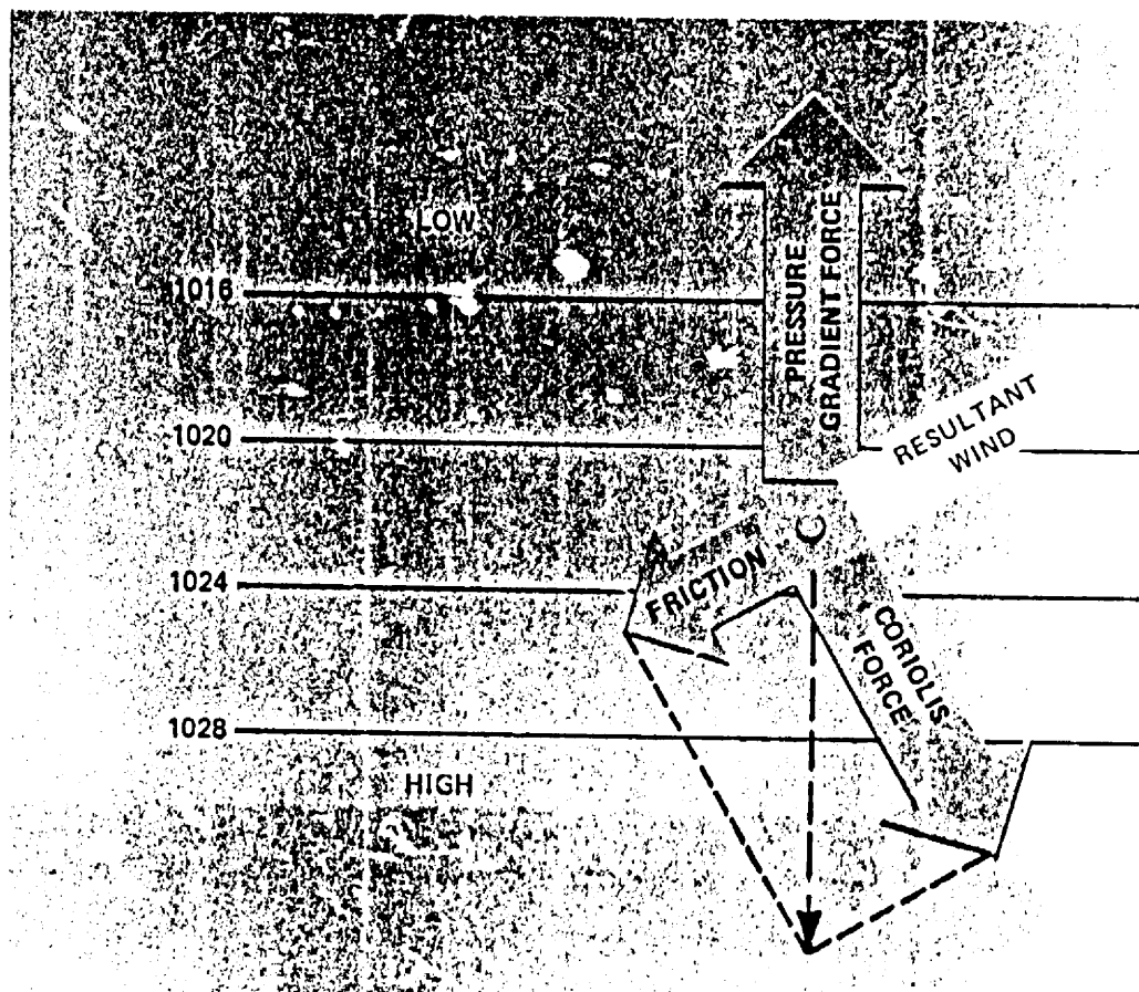
FIGURE 27. Surface friction slows the wind and reduces Coriolis force but does not affect pressure gradient force; winds near the surface are deflected across the isobars toward lower pressure.
