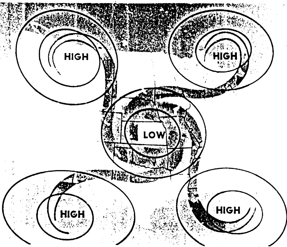
FIGURE 28. Circulation around pressure systems at the surface. Wind spirals outward from high pressure and inward to low pressure, crossing isobars at an angle.
