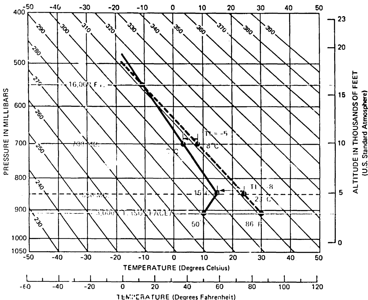
FIGURE 163. Another example of computing T_1 's and maximum height of thermals. See discussion in caption of figure 162. By the time of maximum heating, excellent lift should be available in lower levels and moderate lift above 10,000 feet. Although thermals should continue to 16,000 feet, you could expect weak lift above 12,000 or 13,000 feet because of the small difference between temperatures in the thermal and in the surrounding air.
