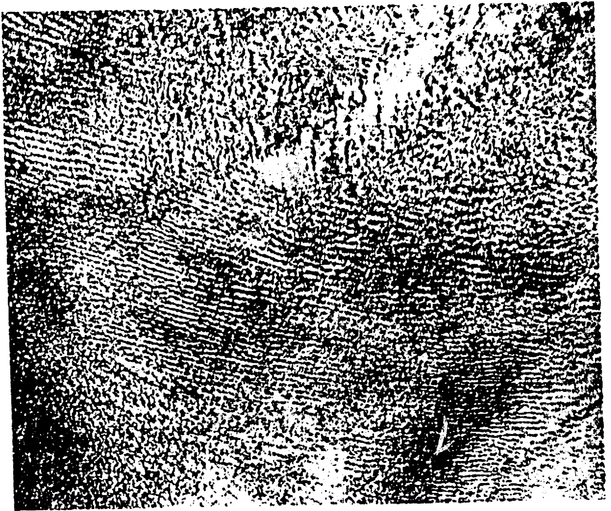
FIGURE 159. Cumulus clouds in thermal streets photographed from a satellite by a high resolution camera. (Courtesy the National Environmental Satellite Service.)
