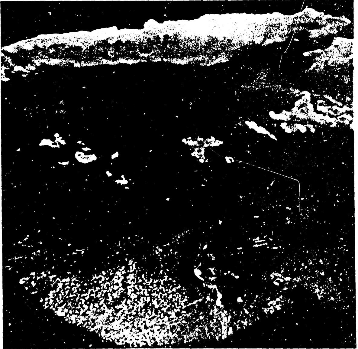
FIGURE 75. An aerial view of a portion of a squall line.
