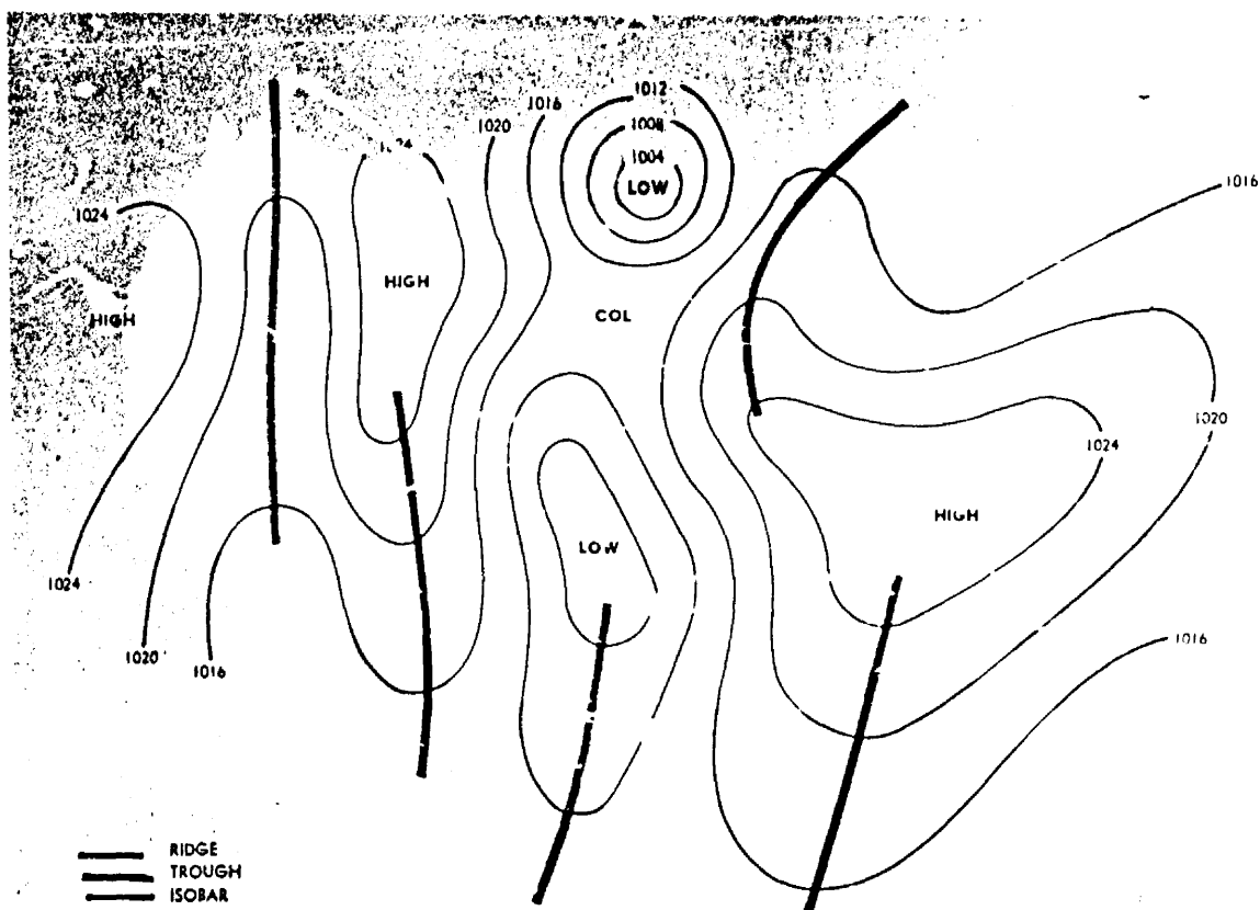
FIGURE 13. Pressure systems.
