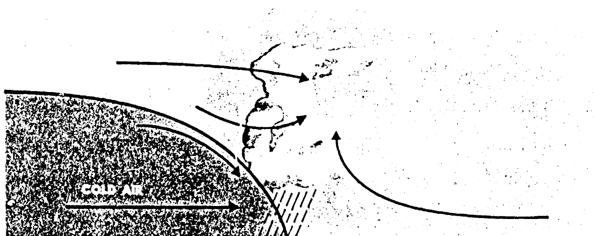
FIGURE 71. A warm front with overrunning warm, moist, unstable air. Weather, clouds, and hazards are similar to those described in figure 70 except that they generally are more widespread.
