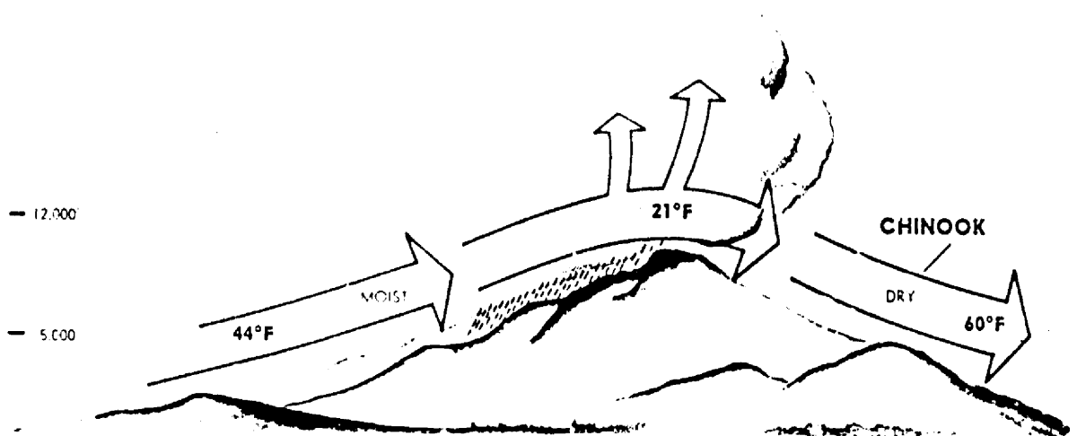
FIGURE 29. The "Chinook" is a katabatic (downslope) wind. Air cools as it moves upslope and warms as it blows down-slope. The Chinook occasionally produces dramatic warming over the plains just east of the Rocky Mountains.
